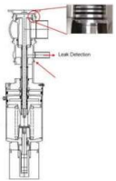
W72RS Series - Double Seat Mix Proof Tank Outlet Valves
