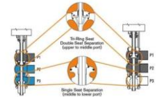
W73 Series - Double Seat Mix Proof Divert Valves
