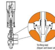
W71 Series - Double Seat Mix Proof Shut-Off Valves
